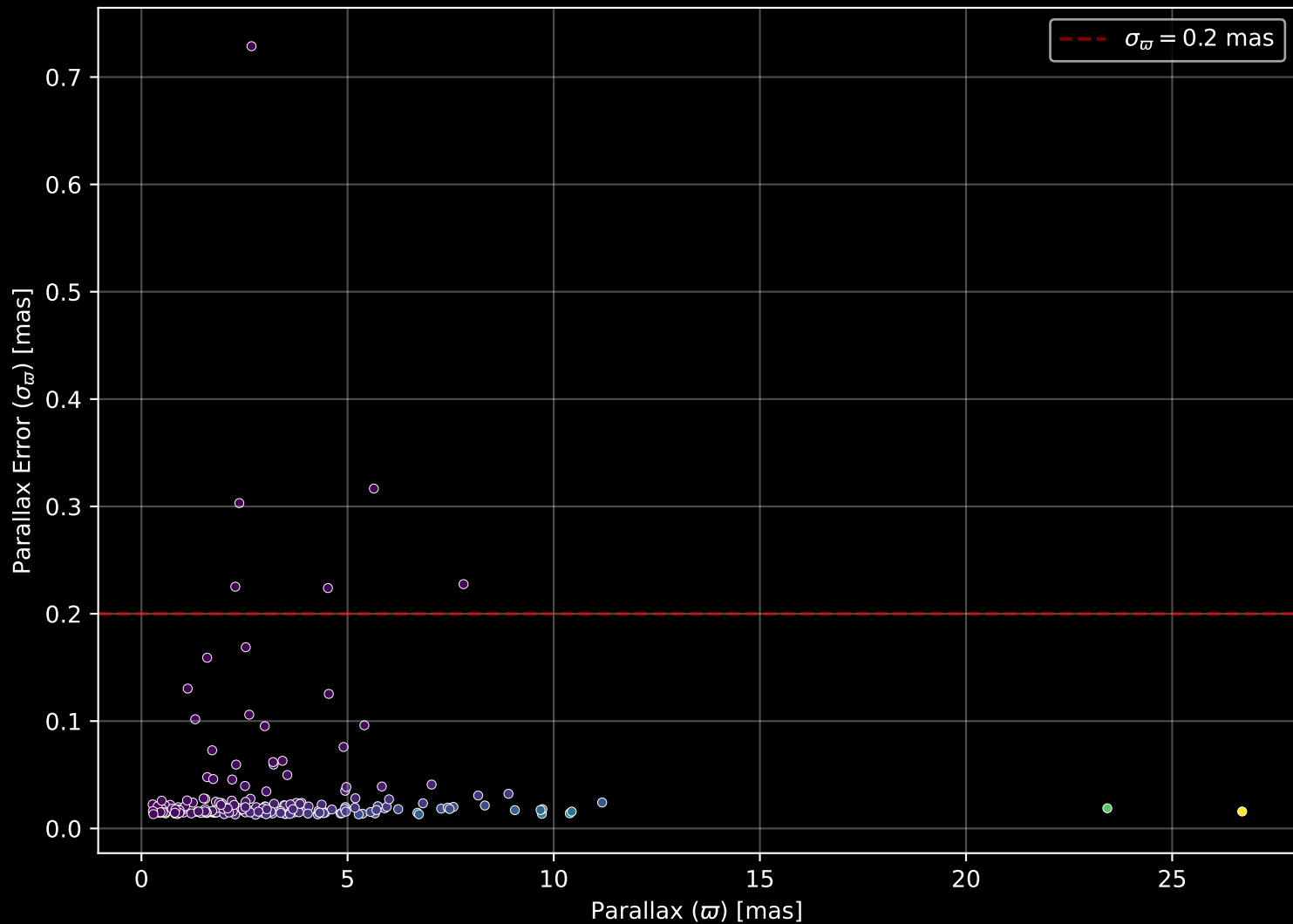
APOGEE DR17 Field: [192-47_MGA] Parallax Quality (n= 206)
