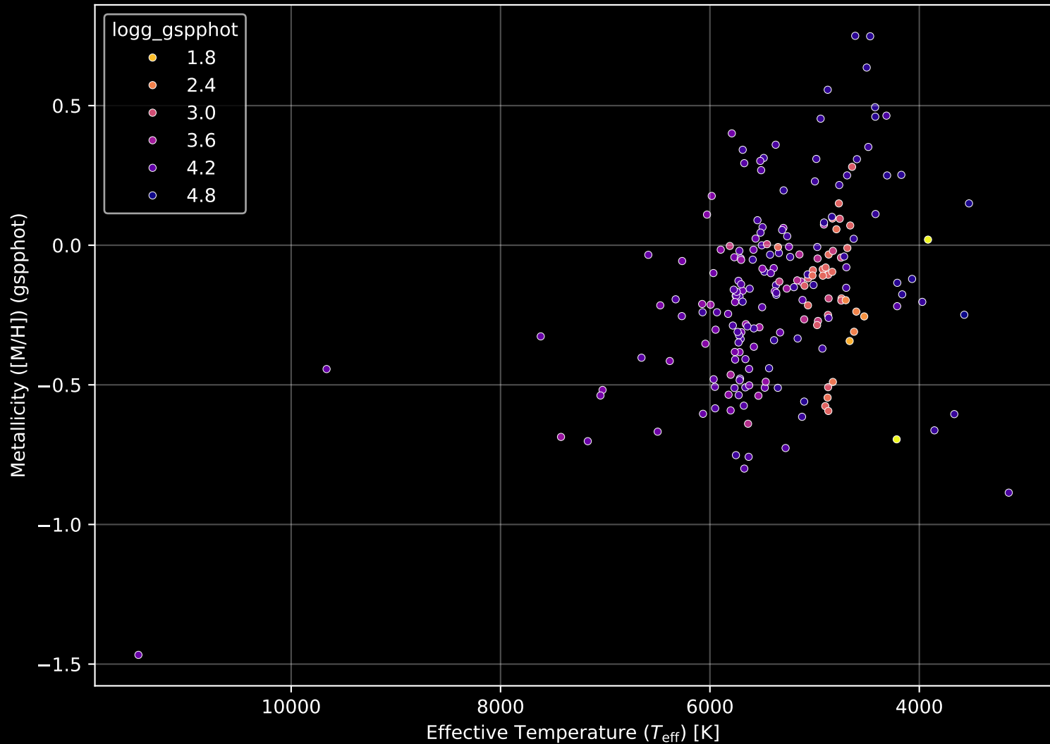
APOGEE DR17 Field: [192-47_MGA] Stellar Population Parameters (n= 206)
